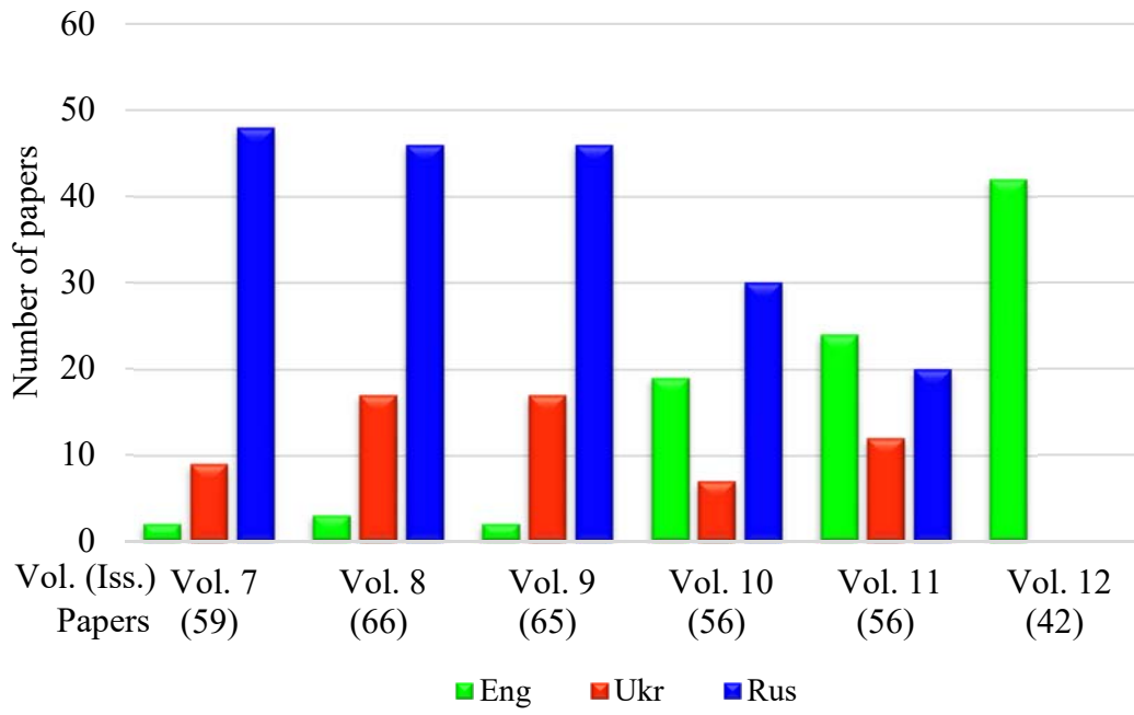
Languages of papers by Volumes (years)
