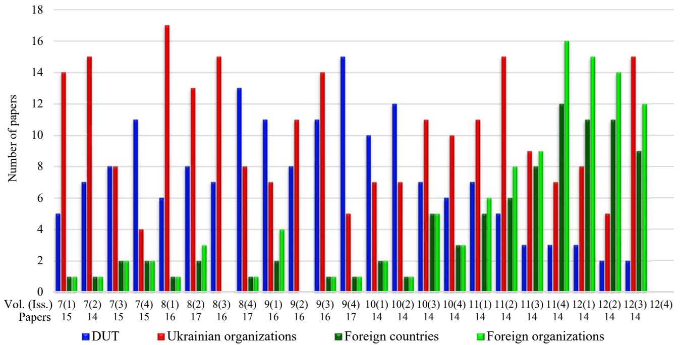
Papers of DUT employee vs Ukrainian organizations and Foreign countries by Issues
