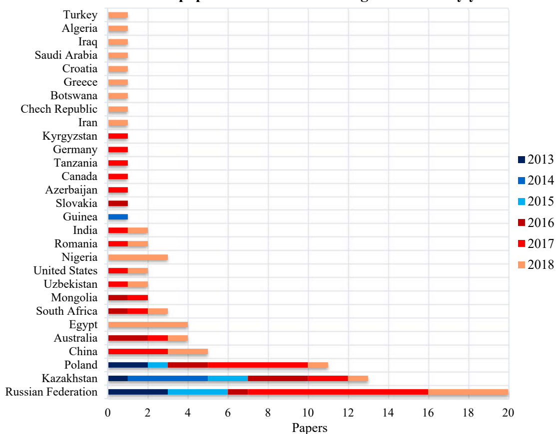
Number of papers affiliated with foreign countries by years
