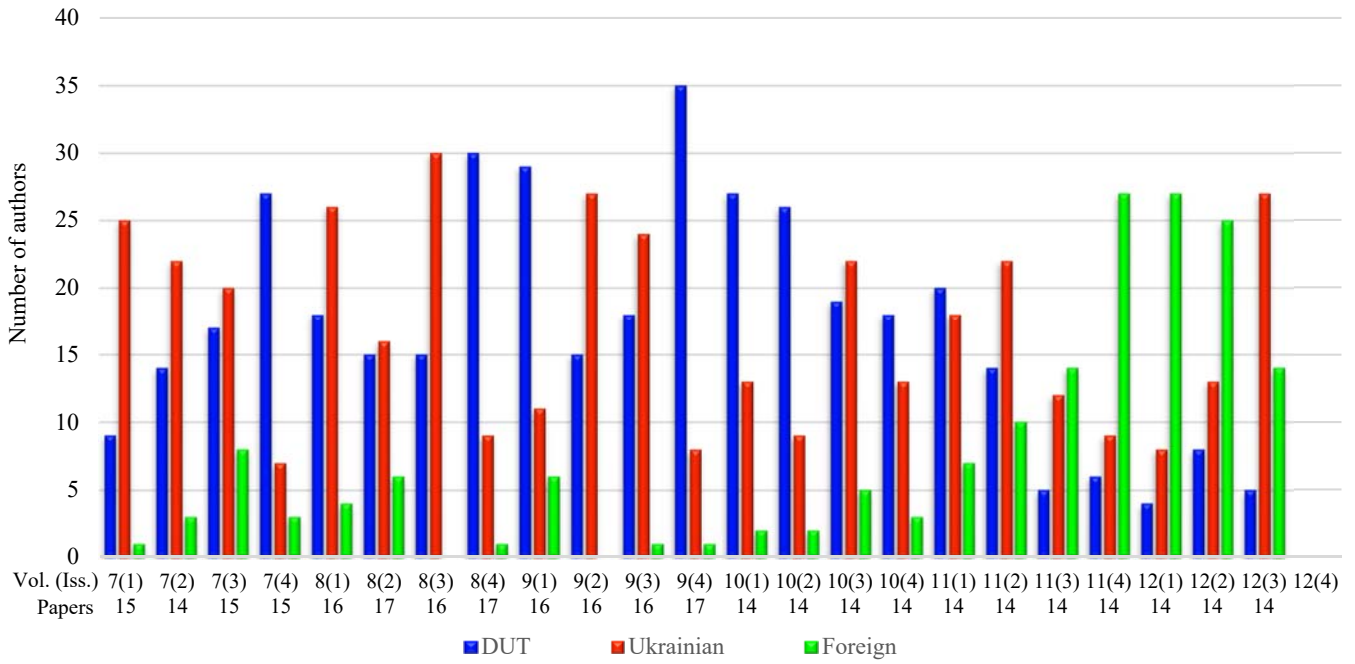
Number of DUT authors vs Ukrainian and Foreign authors by Issues
