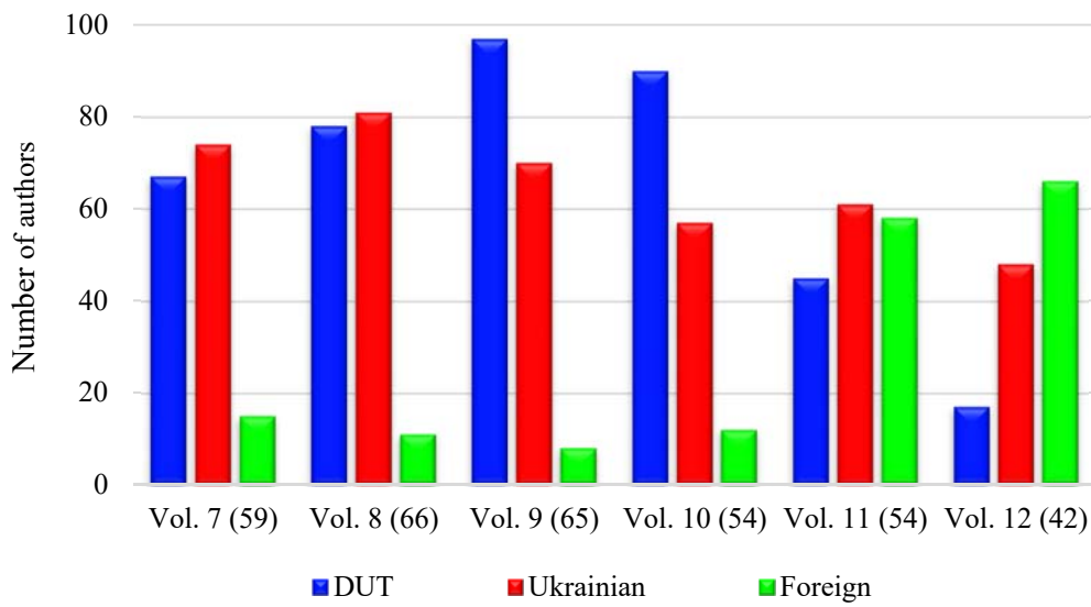
Number of DUT authors vs Ukrainian and Foreign authors, by Volumes (years)
