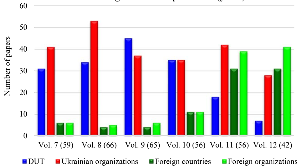
Papers of DUT employee vs Ukrainian organizations and Foreign countries by Volumes (years)
